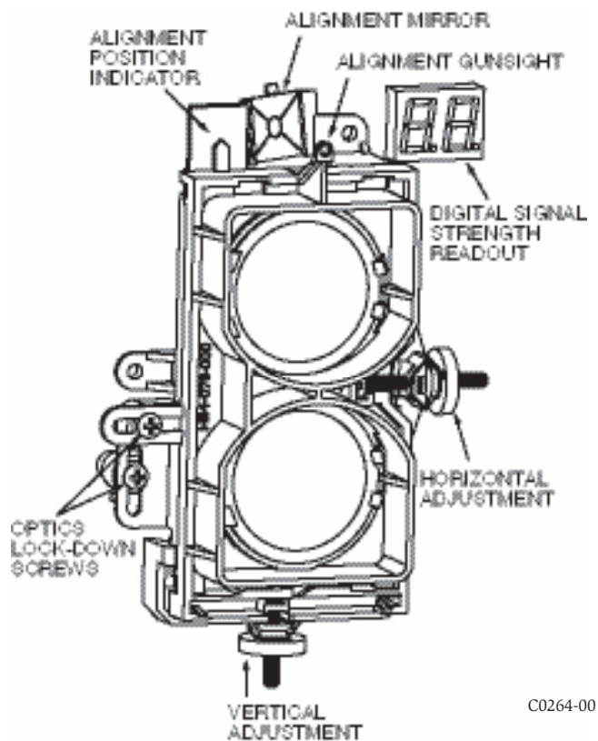
FIGURE 11. ALIGNMENT ADJUSTMENT LOCATIONS
