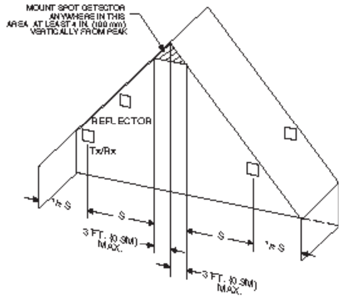
FIGURE 4. SLOPED CEILING (PEAKED TYPE):
