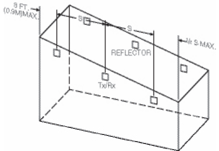
FIGURE 4. SLOPED CEILING (PEAKED TYPE):
