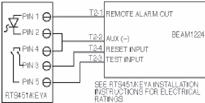
FIGURE 8. WIRING DIAGRAM (RTS451)
