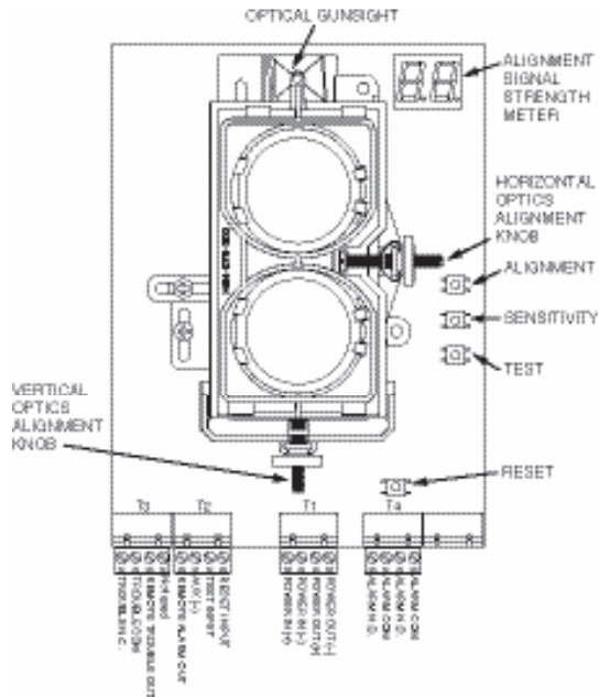
FIGURE 6. WIRING CONNECTIONS AT DETECTOR
